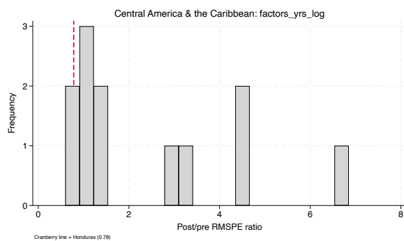
factors_yrs_log
