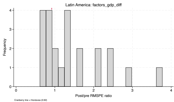
factors_gdp_diff
