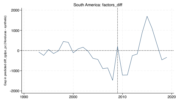
factors_diff
