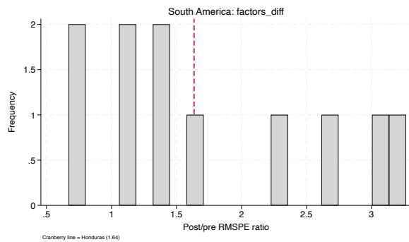
factors_diff
