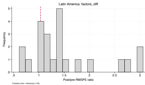
factors_diff
