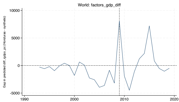
factors_gdp_diff
