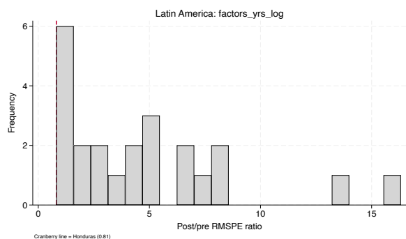
factors_yrs_log
