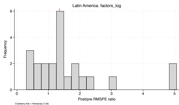
factors_log
