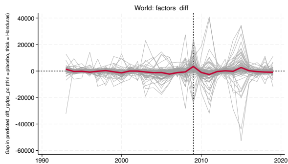
factors_diff
