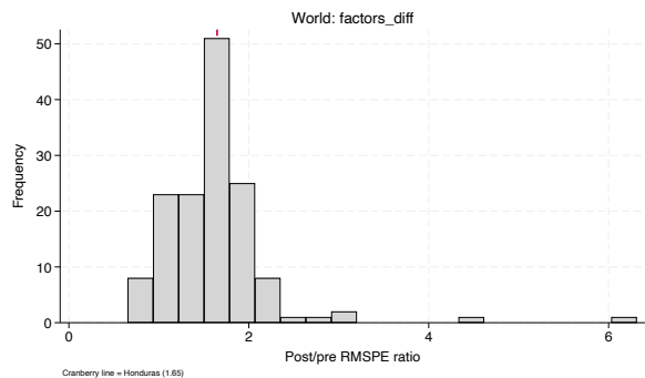
factors_diff
