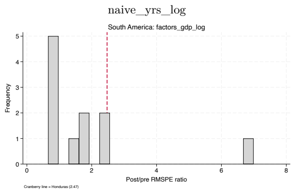
factors_gdp_log
