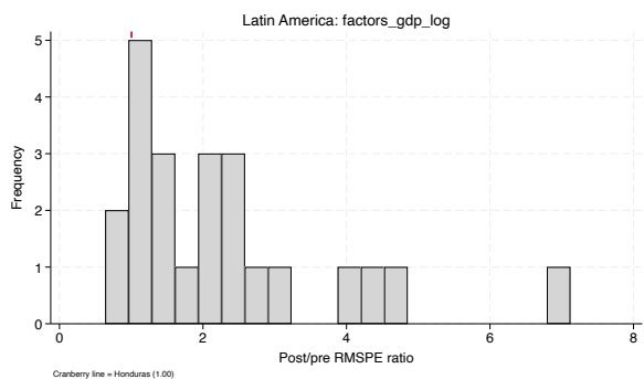
factors_gdp_log
