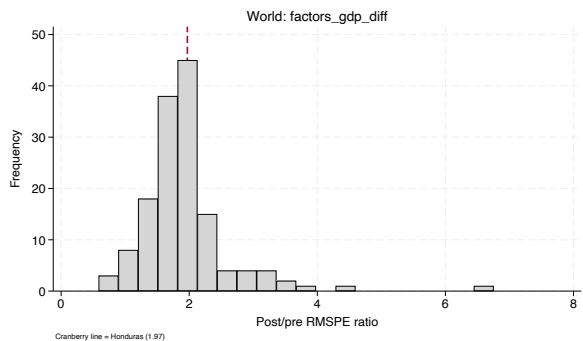
factors_gdp_diff
