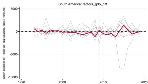
factors_gdp_diff
