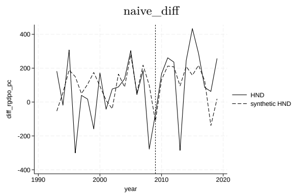
factors_gdp_diff
