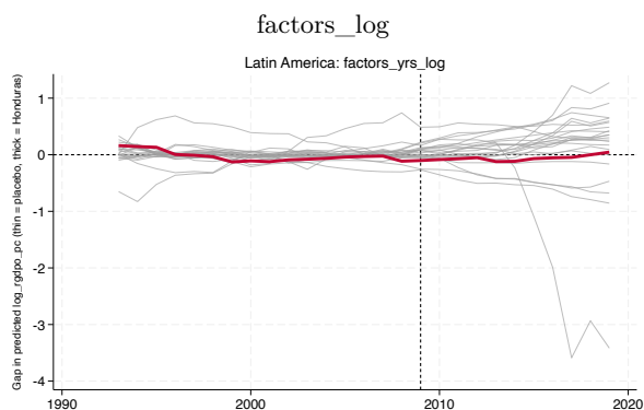
factors_yrs_log
